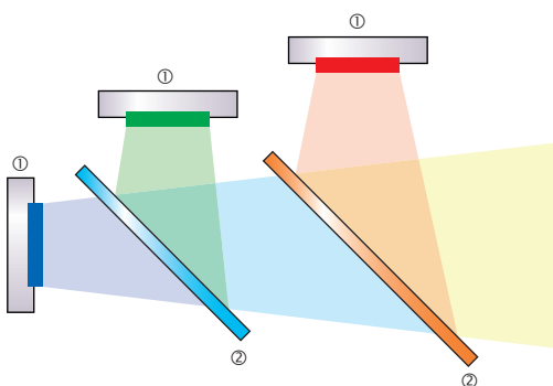
① LED Source ② LED ColorDichroics™
