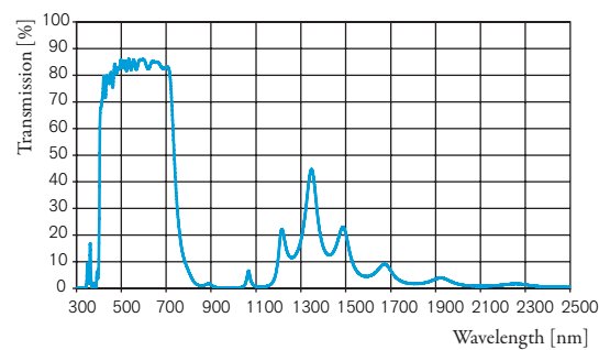
Spectral performance of the Calflex™ 3000 SP
