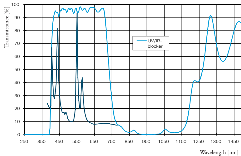
Spectral curve of UV/IR-blocker and emission spectrum of typical projection lamp
